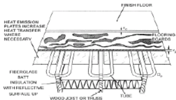
Tube under Subfloor
