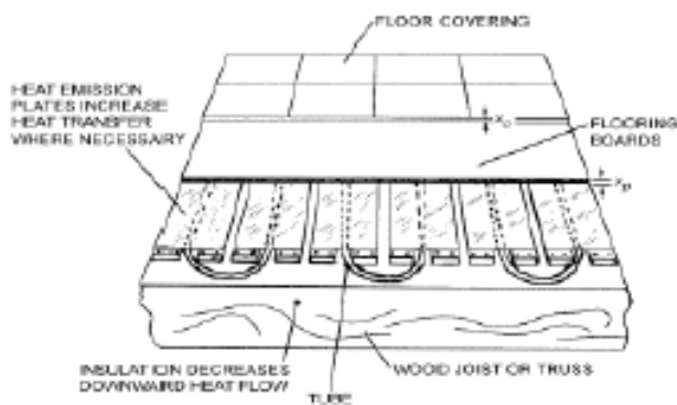
Tube in Subfloor
